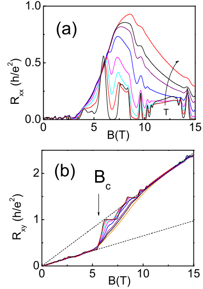
FIG. 3. (Color online) (a) Longitudinal and Hall resistances of a parabolic quantum well with disordered superlattice (sample E) for different temperatures T (from top to bottom): 950 mK (red), 750 mK (black), 700 mK (purple), 520 mK (blue), 475 mK (magenta), 320 mK (cyan), 240 mK (red), and 90 mK (black). (b) Filling factors determined from the Hall resistance are labeled. The dashed line corresponds to the linear extrapolation of the low-field Hall resistance. Arrow shows the critical magnetic field when transition occurs.
