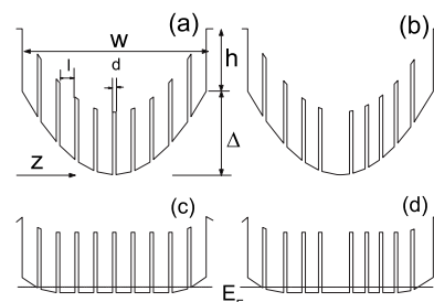
FIG. 1. The profile of the conduction-band edge of an (a) and (b) empty and (c) and (d) partially filled parabolic well with (a) and (c) periodic and (b) and (d) intentionally disordered superlattices. E_F is the Fermi level.
