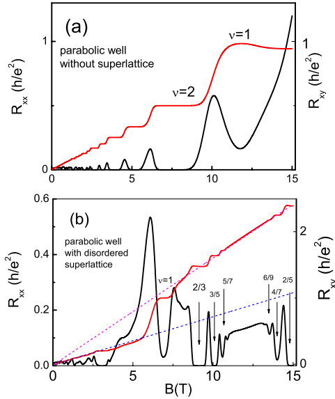
FIG. 2. (Color online) Longitudinal (black) and Hall (red) resistances as functions of the perpendicular magnetic field for a parabolic quantum well (a) without superlattice (sample A) and (b) with disordered superlattice (sample E). Filling factors determined from the Hall resistance are labeled. FQH states are marked with arrows. The dashed lines correspond to the linear extrapolation of the low-field and high-field Hall resistances.
